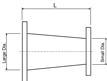
Concentric Reducer
