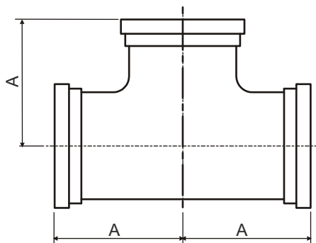
Shouldered Equal Tee
