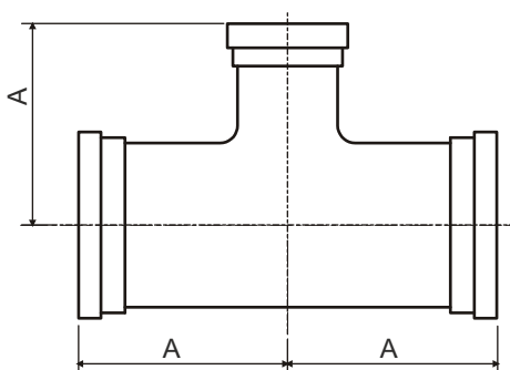
Shouldered Tee
