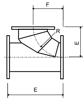
Short Radius 1D
